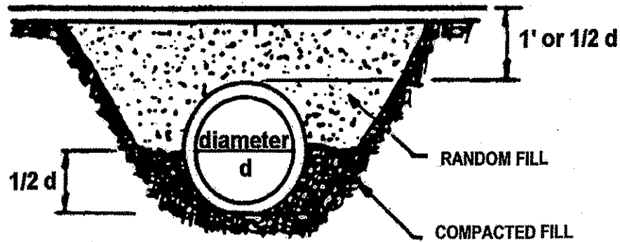
Figure 4-9a. Typical Culvert Installation
