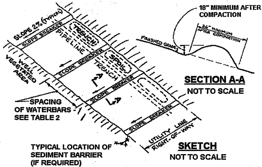
FIGURE 32 Waterbar Installation
