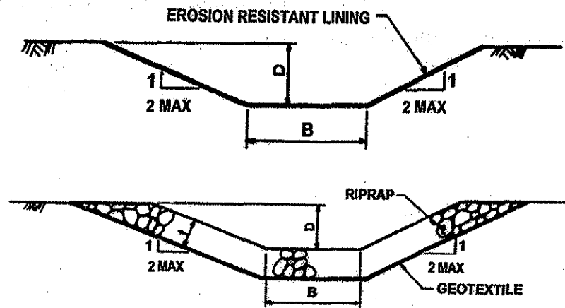
Figure 4-2. Typical Channel Cross Sections
