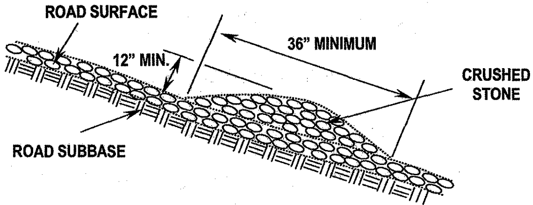
Figure 4-11. Waterbar Dimensions
