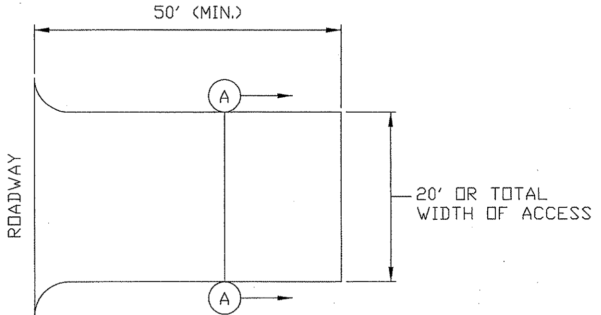
PLAN VIEW
