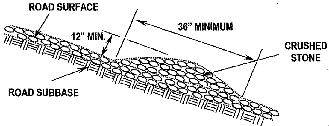
Figure 4-11. Waterbar Dimensions
