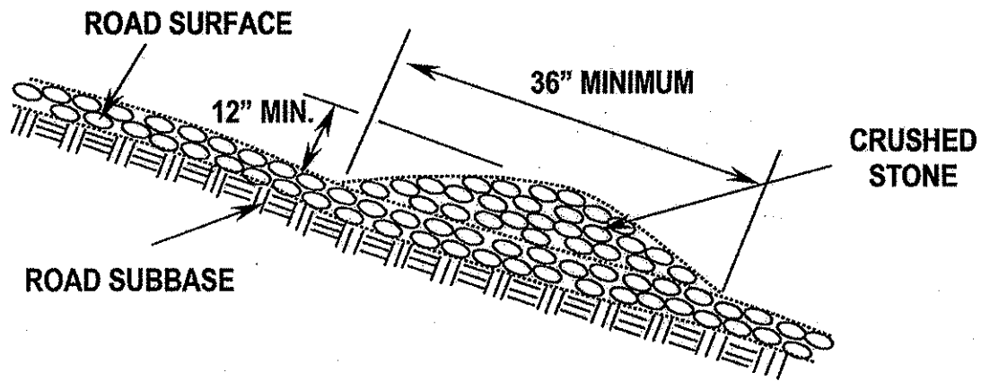
Figure 4-11. Waterbar Dimensions
